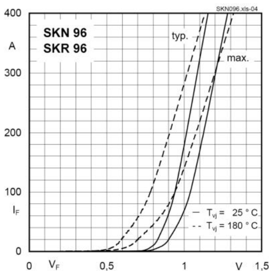
Fig. 5 Forward characteristics
